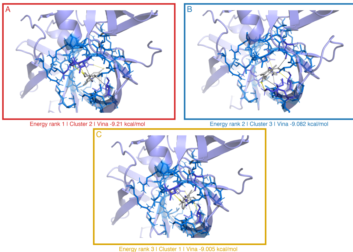
Figure 3. Three-dimensional interaction snapshots for Rilpivirine. Shown are 3 energy-ranked distinct cluster representatives, ordered by Vina score. Panels A, B, and C show energy ranks 1, 2, and 3, respectively. Red, blue, and gold match the highlighted clusters in Figure 2. These views support structural inspection; docking score rank does not establish pose correctness.
