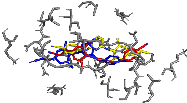
Figure 2. Docking pose-cluster analysis for Rilpivirine. (A) Docking score versus symmetry-aware, no-fit heavy-atom RMSD from the lowest-energy cluster representative in the receptor coordinate frame; point size denotes cluster population. (B) Representative structures from the highlighted clusters, using matching cluster colors. Gray protein residues are the residues within 5 Å of the displayed representative ligands.
