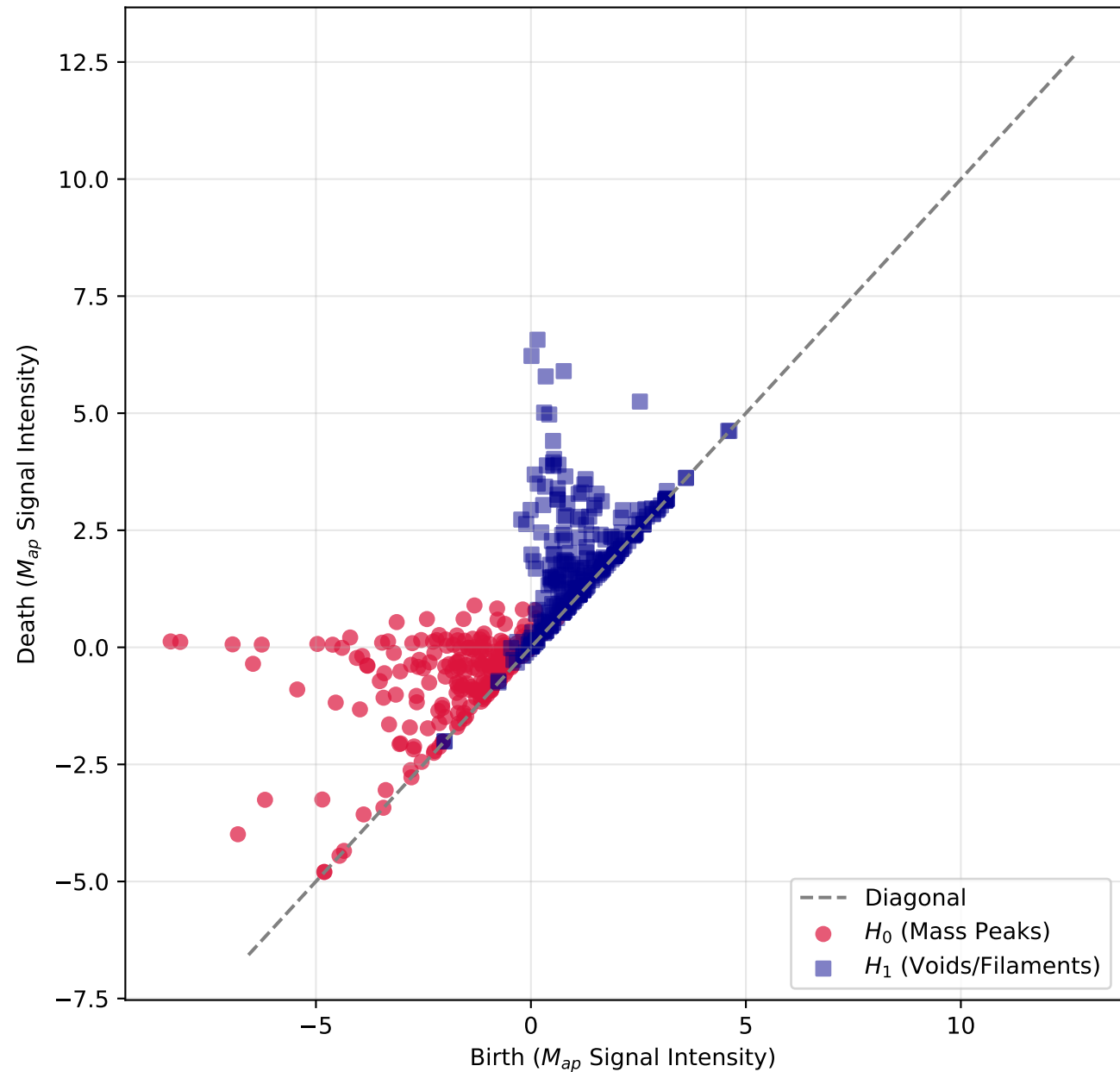
Superlevel Set Persistence Diagram
