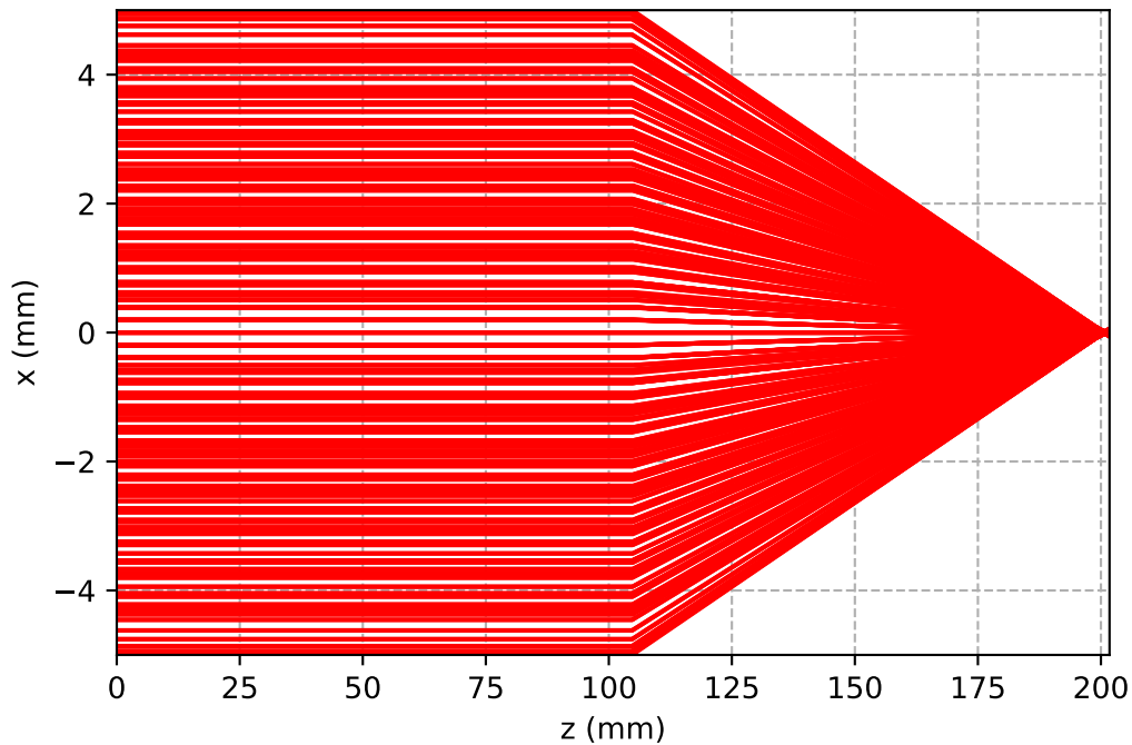
Ray Propagation for y = 0 mm
