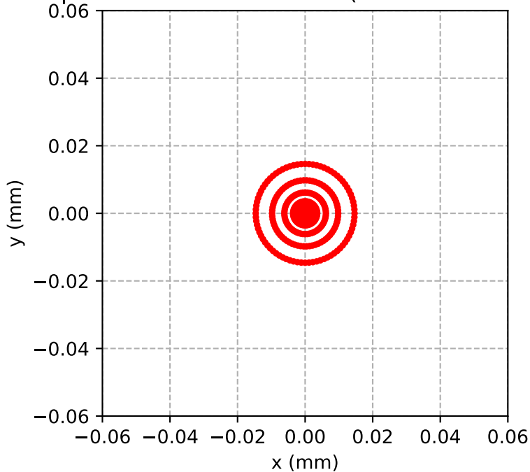
Output Plane at z = 198 mm (Paraxial Focal Plane)
