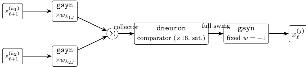
Figure 6: Sign-faithful backward (BKSIGN), one hidden neuron j of layer \ell . The children’s errors are weighted by the (shared) weight capacitors, summed as currents, regenerated to a clean sign by a saturating comparator, and injected into the value node. Error alignment survives depth as a sign even when magnitudes cannot.
