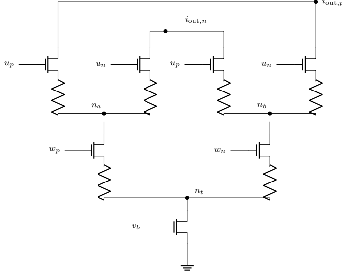
Figure 1: Synapse gsyn (7 NMOS + 6 source-degeneration resistors, all 12 k \Omega ; tail 400/100, all others 200/100 \mu\text{m} ). The weight pair (gates w_p, w_n ) splits the tail current between branch rails n_a, n_b ; the cross-coupled input quad (gates u_p, u_n ) steers each branch to the two output wires ( u_p pulls i_{\text{out},p} from the n_a side but i_{\text{out},n} from the n_b side—that crossing is the multiply). Result: I_{\text{out}} \approx -G \tanh(2.25u) \tanh(k_w w) , G \approx 0.105 . Output is a current , so many synapses sum on a wire for free (fact 2). Mind the sign inversion.
