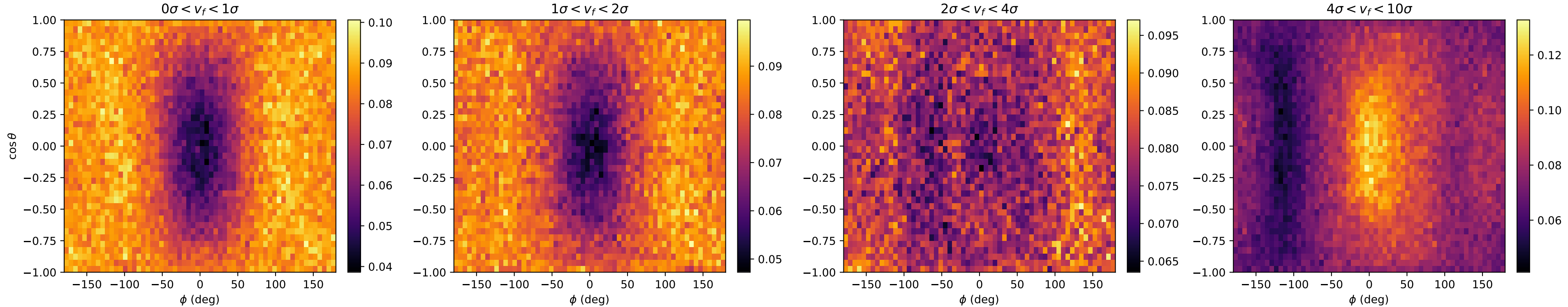
Conditional angular distribution | q=0.01 , e=0.90 , a/a_h=0.1
