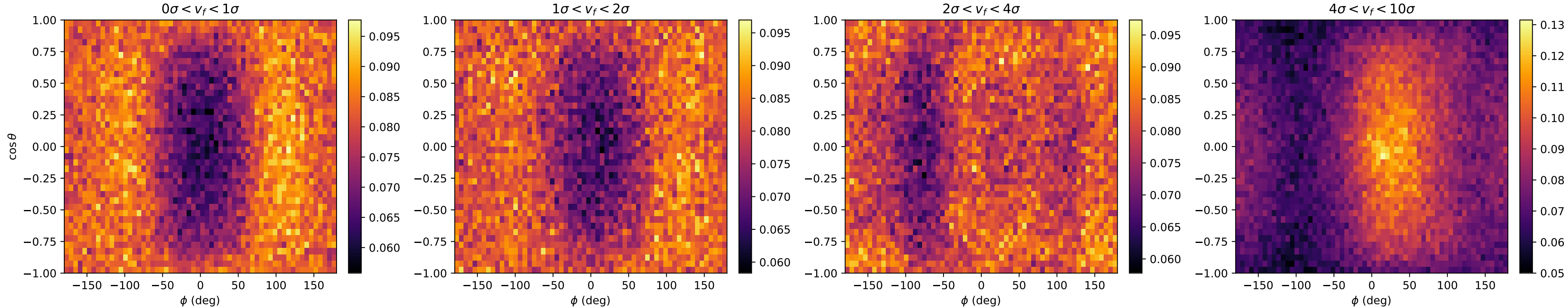
Conditional angular distribution | q=0.2 , e=0.60 , a/a_h=0.1
