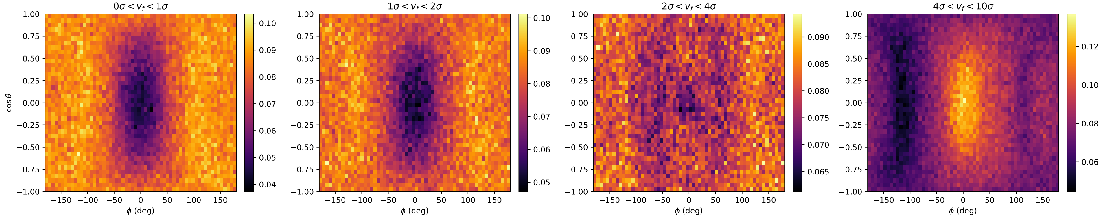
Conditional angular distribution | q=0.001 , e=0.90 , a/a_h=0.1
