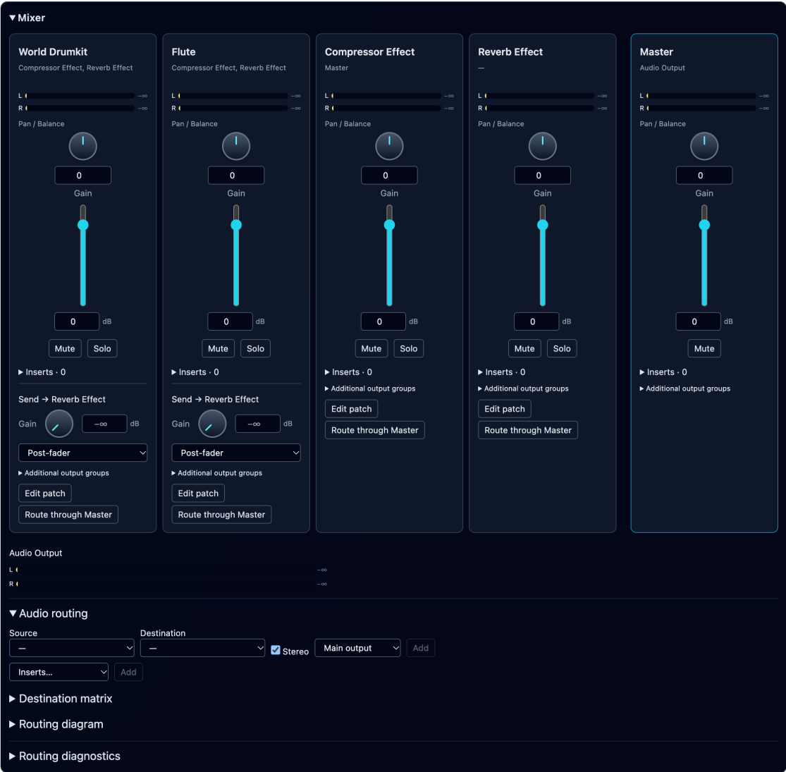
Live “Ratchet drums demo” mixer, stopped: the strips follow the rack’s grouped order, with Master pinned at the right. World Drumkit and Flute have post-fader send controls for Reverb Effect; both sends are set to silence ( -\infty dB). This performance has no insert processors.
