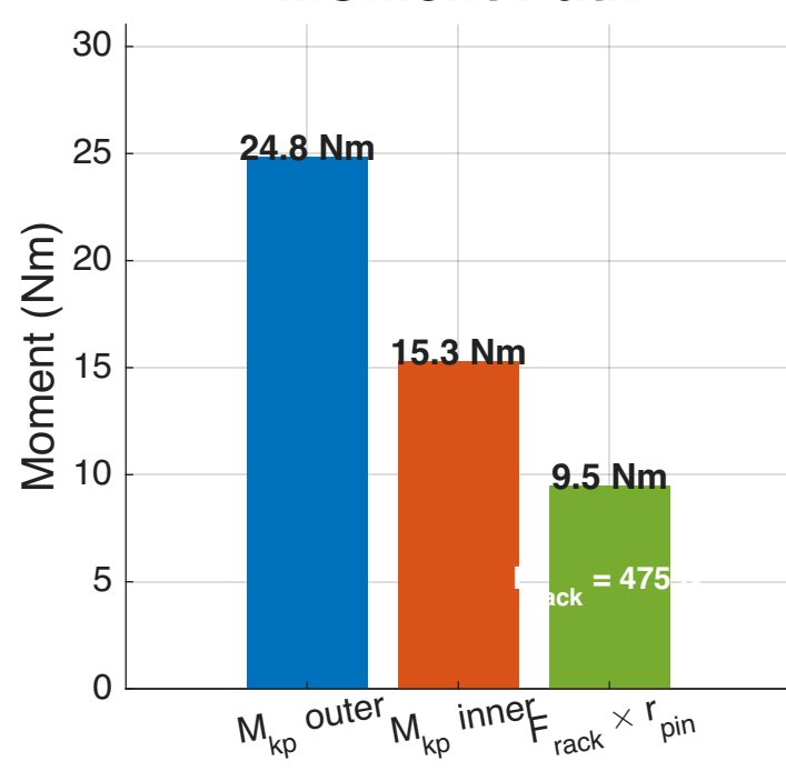
Moment Path
