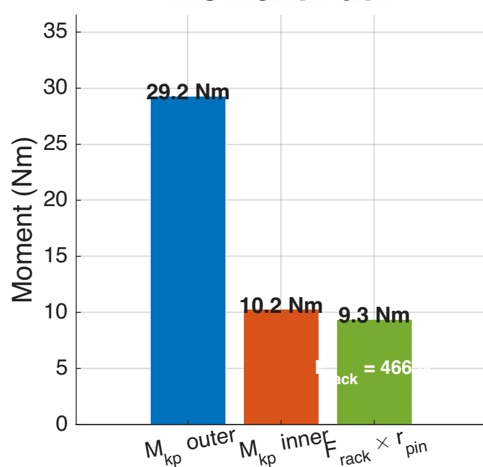
Moment Path
