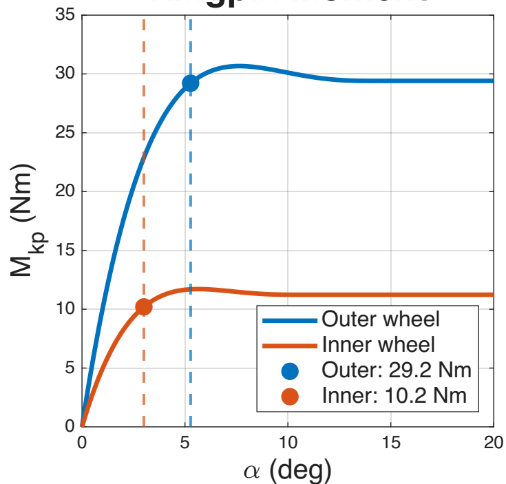
Kingpin Moment
