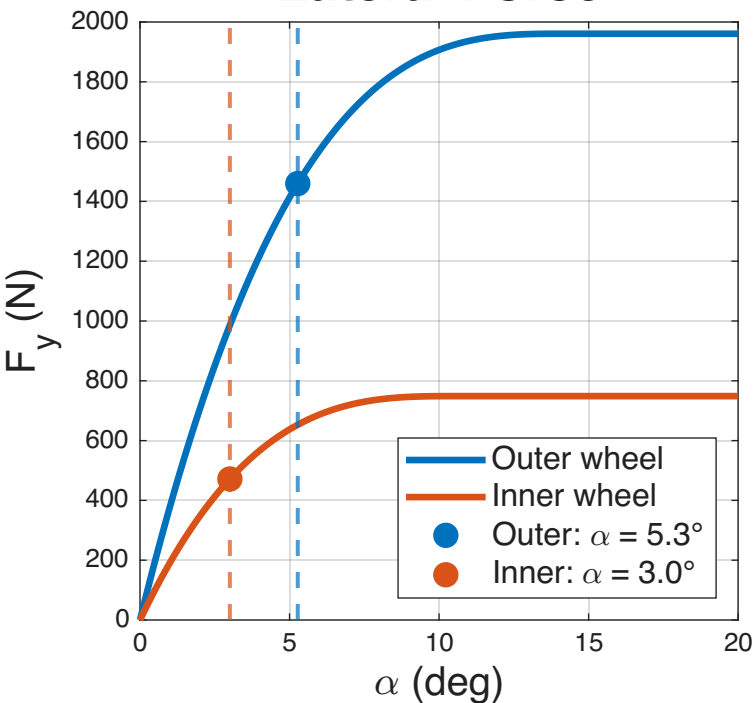
Lateral Force
