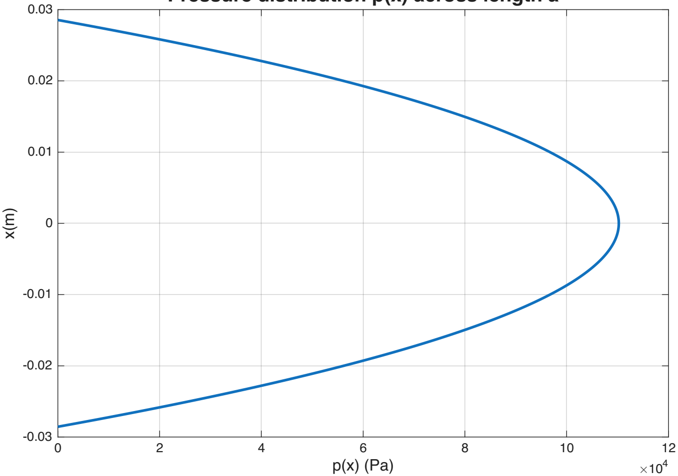
Pressure distribution p(x) across length a
