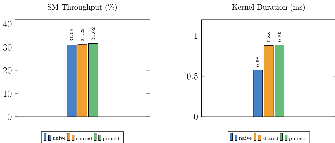
Abbildung 10: NMS-Profilung, SOBEL_OPT=4 (Bucket-Richtung). SM Throughput aus NCU (10 Runs), Kernel Duration aus cudaEvent-Messung (200 Runs Avg).
