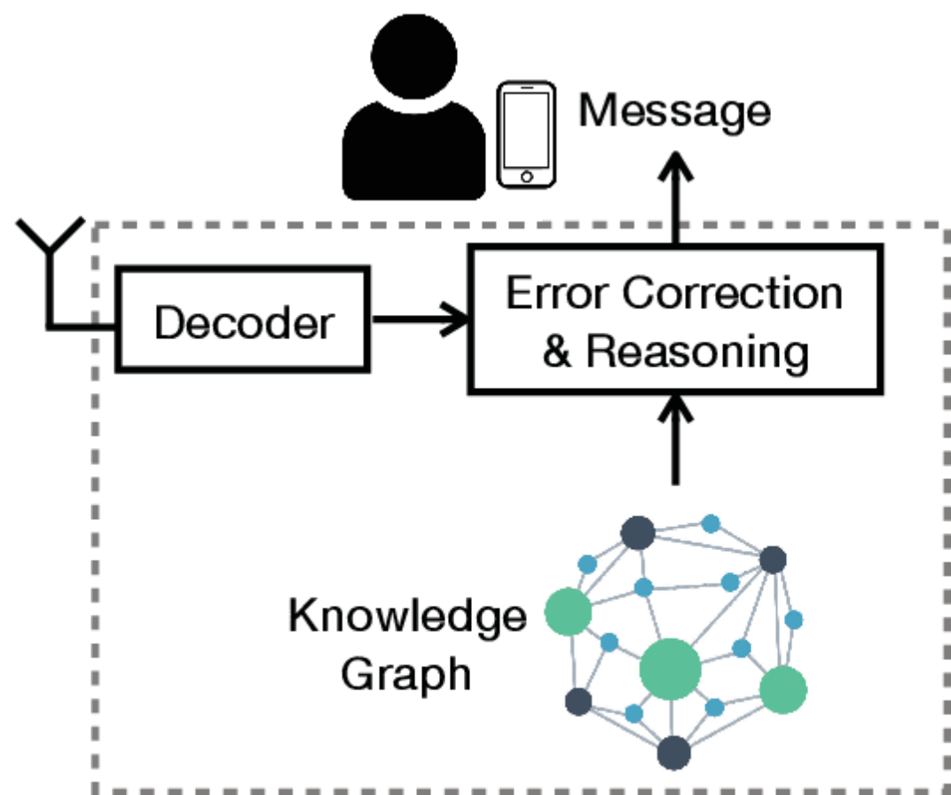
Semantic Decoder
