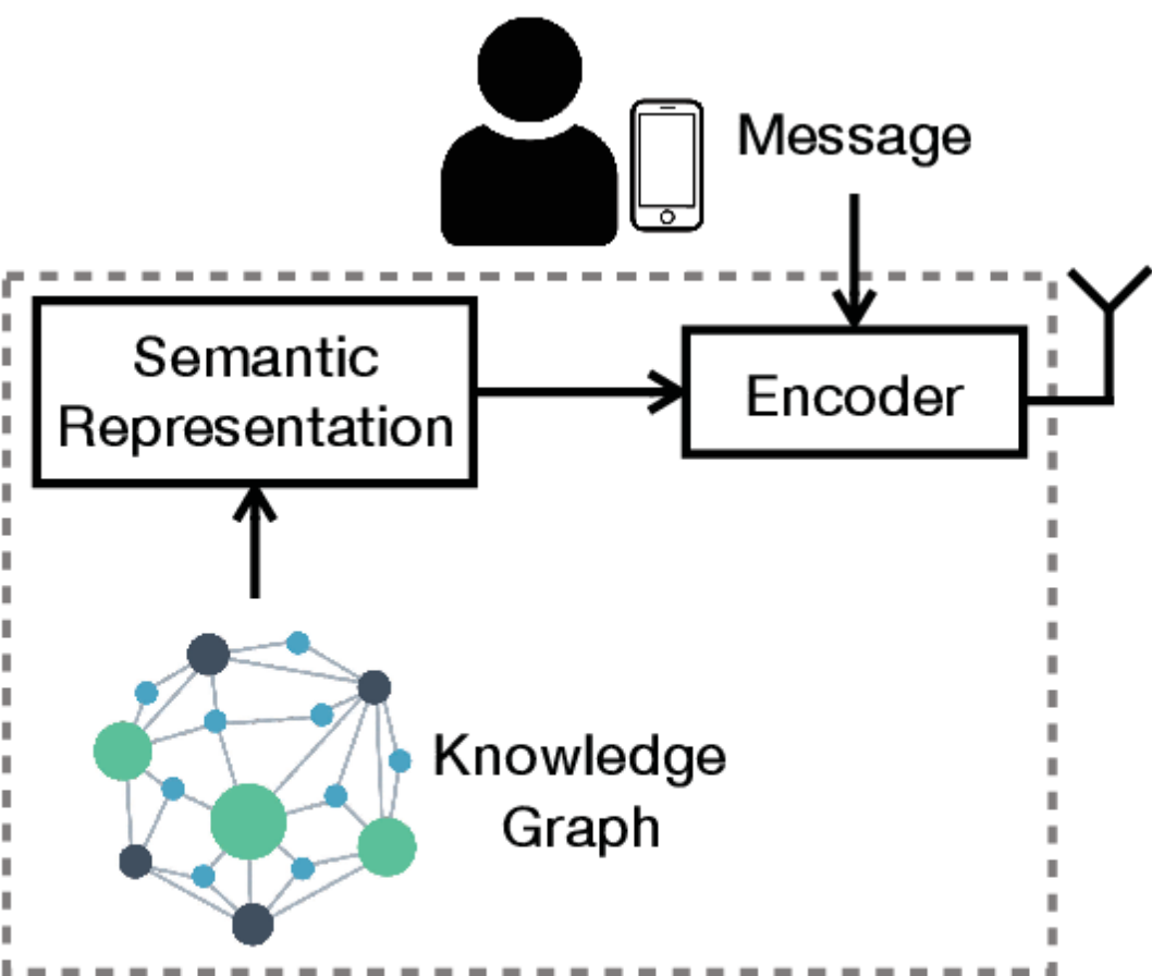
Semantic Encoder
