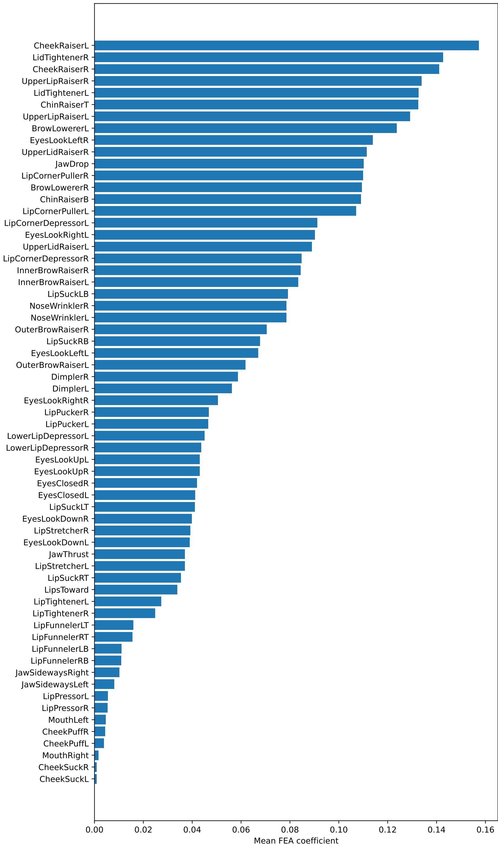
Pooled mean coefficient across all DFEA observations
