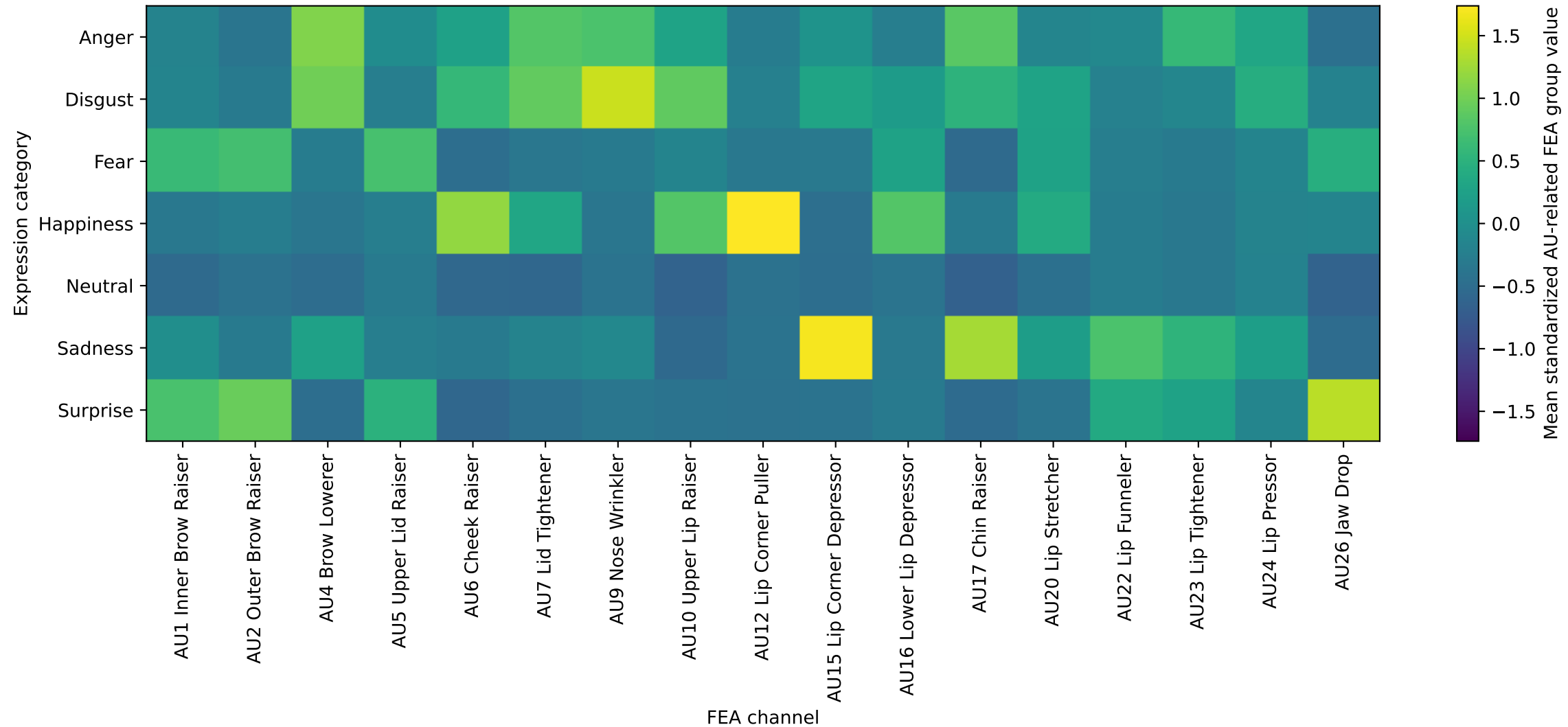
Manuscript AU-related FEA groups — sequence mean, sample-weighted
