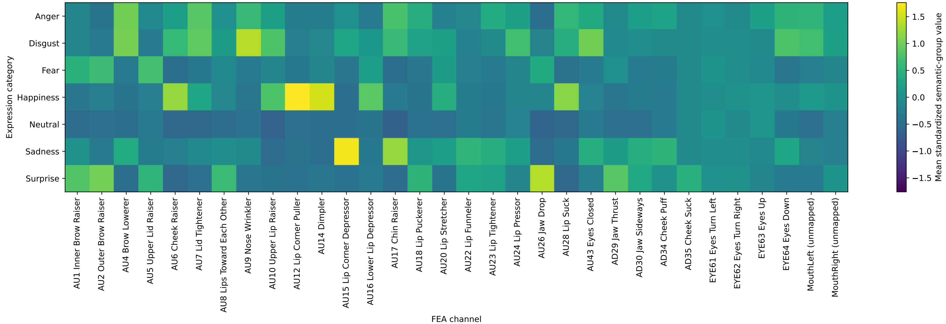
Relative FACS-related FEA groups — sequence mean, participant-balanced
