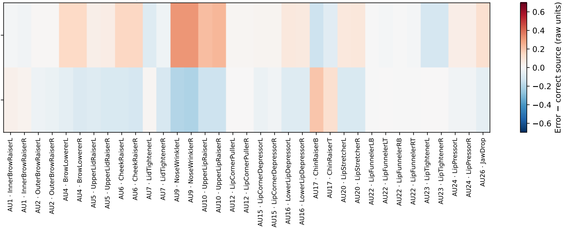
Anger / Disgust: directed errors minus correct source
