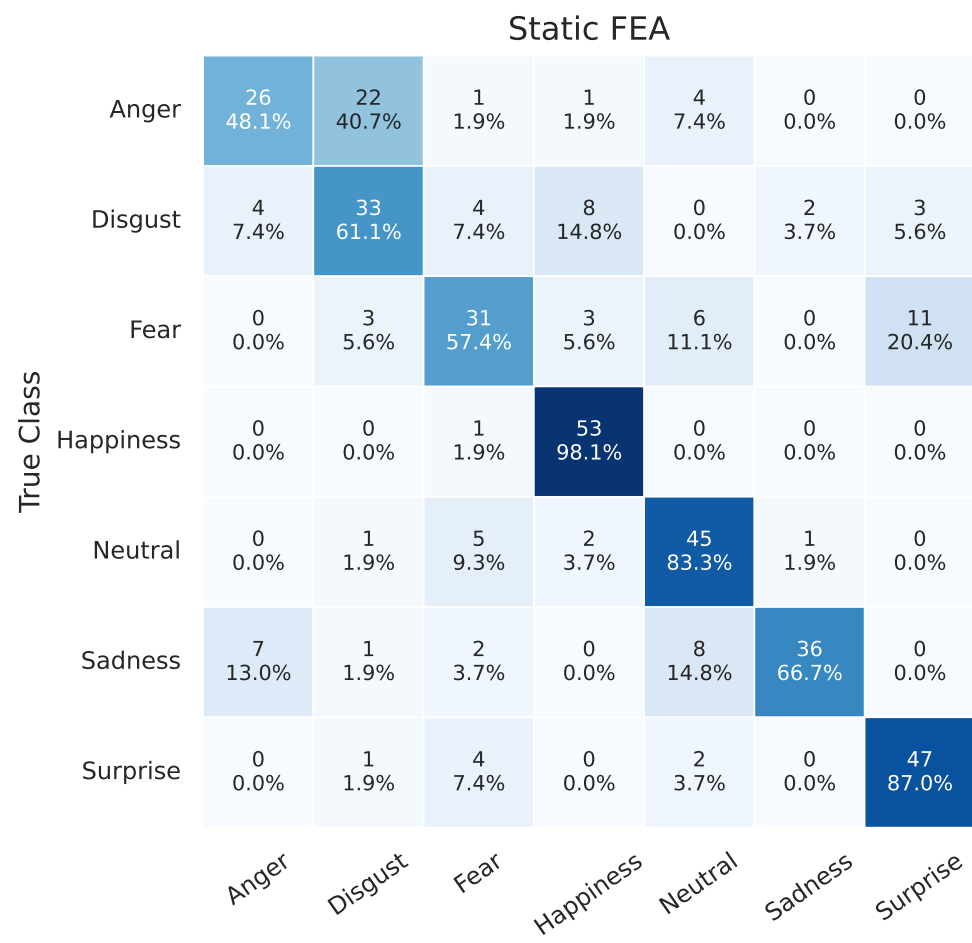
Confusion Matrices: Counts and Row-Normalized Percentages
