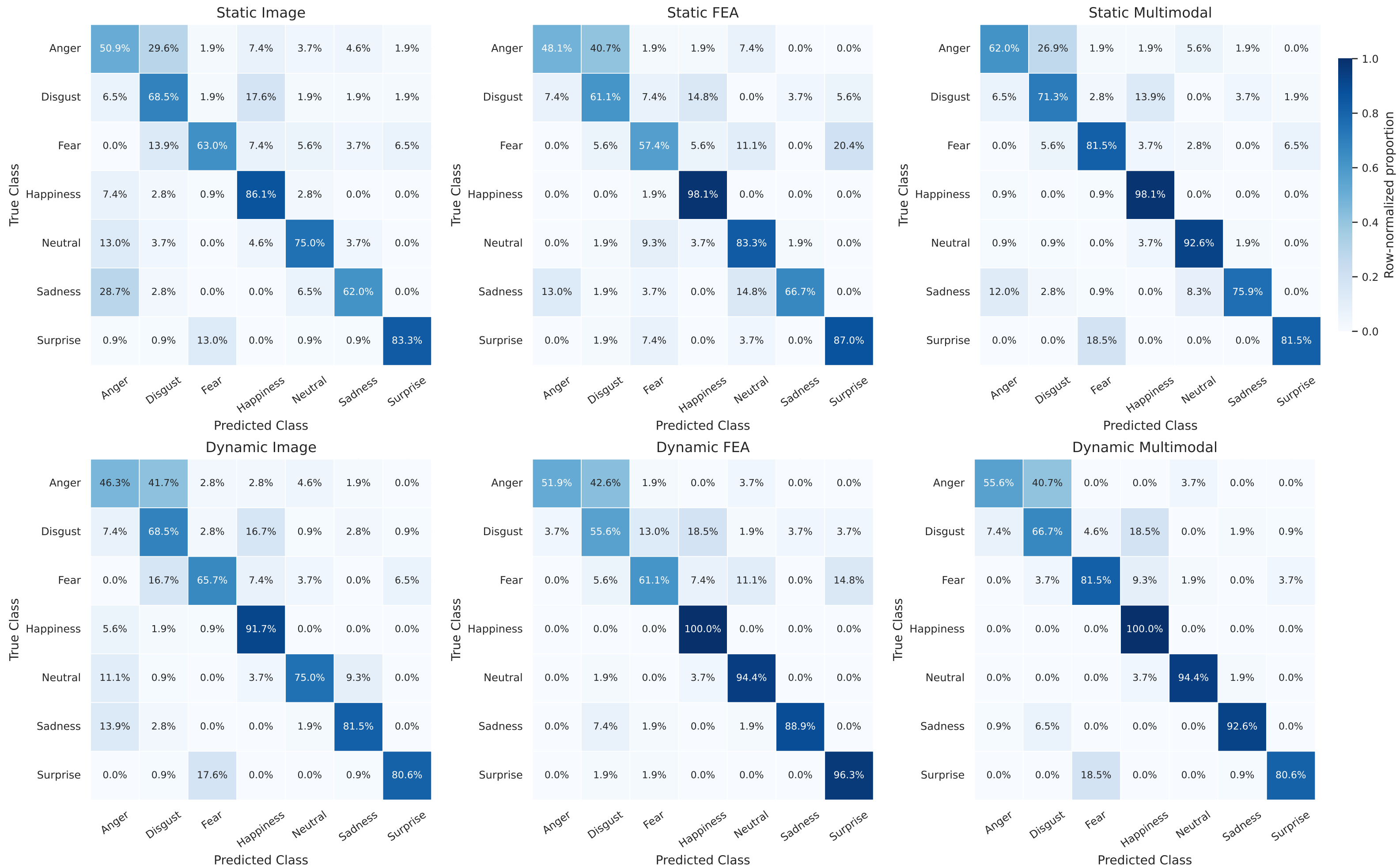
Confusion Matrices: Row-Normalized Percentages
