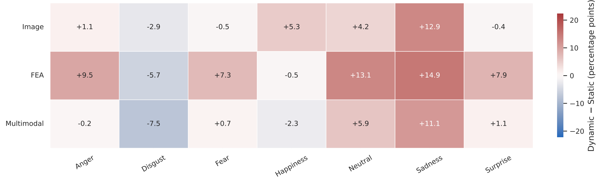
F1-score
