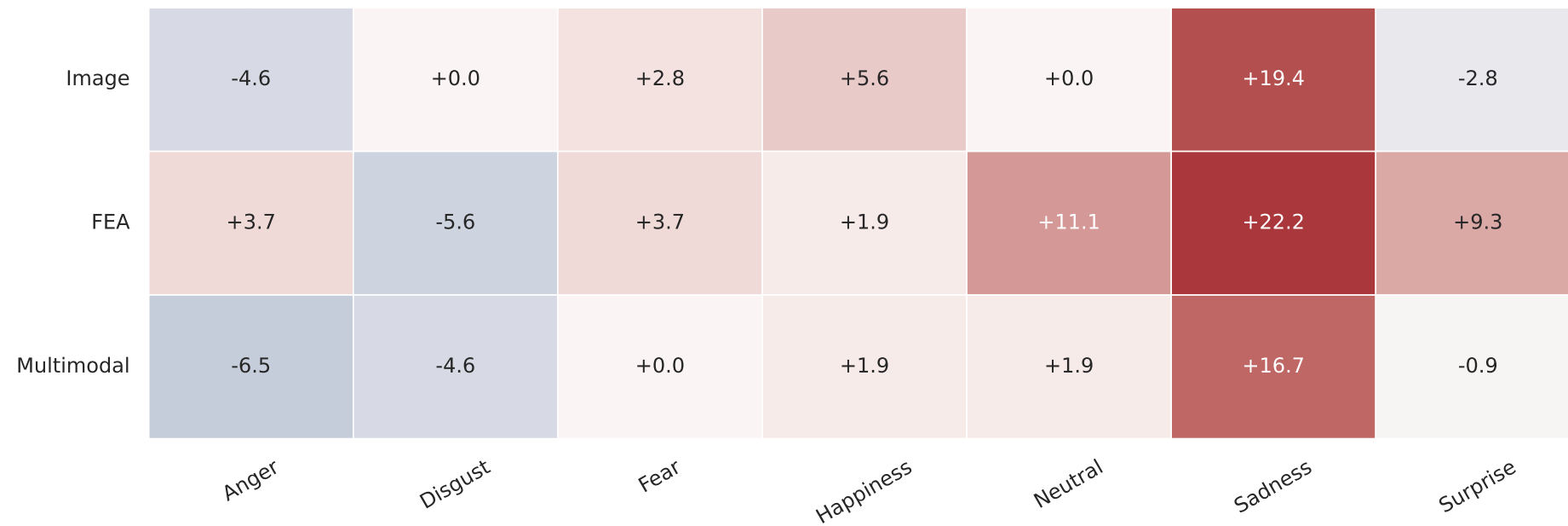
F1-score
