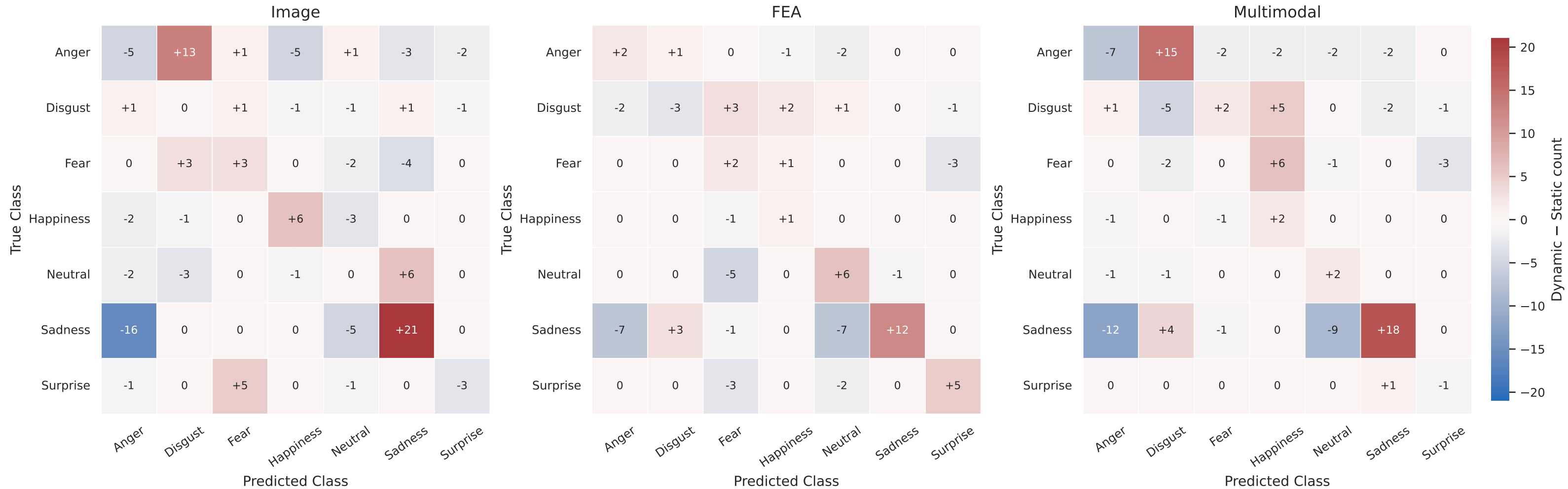
Delta Confusion Matrices: Dynamic – Static (Counts)
