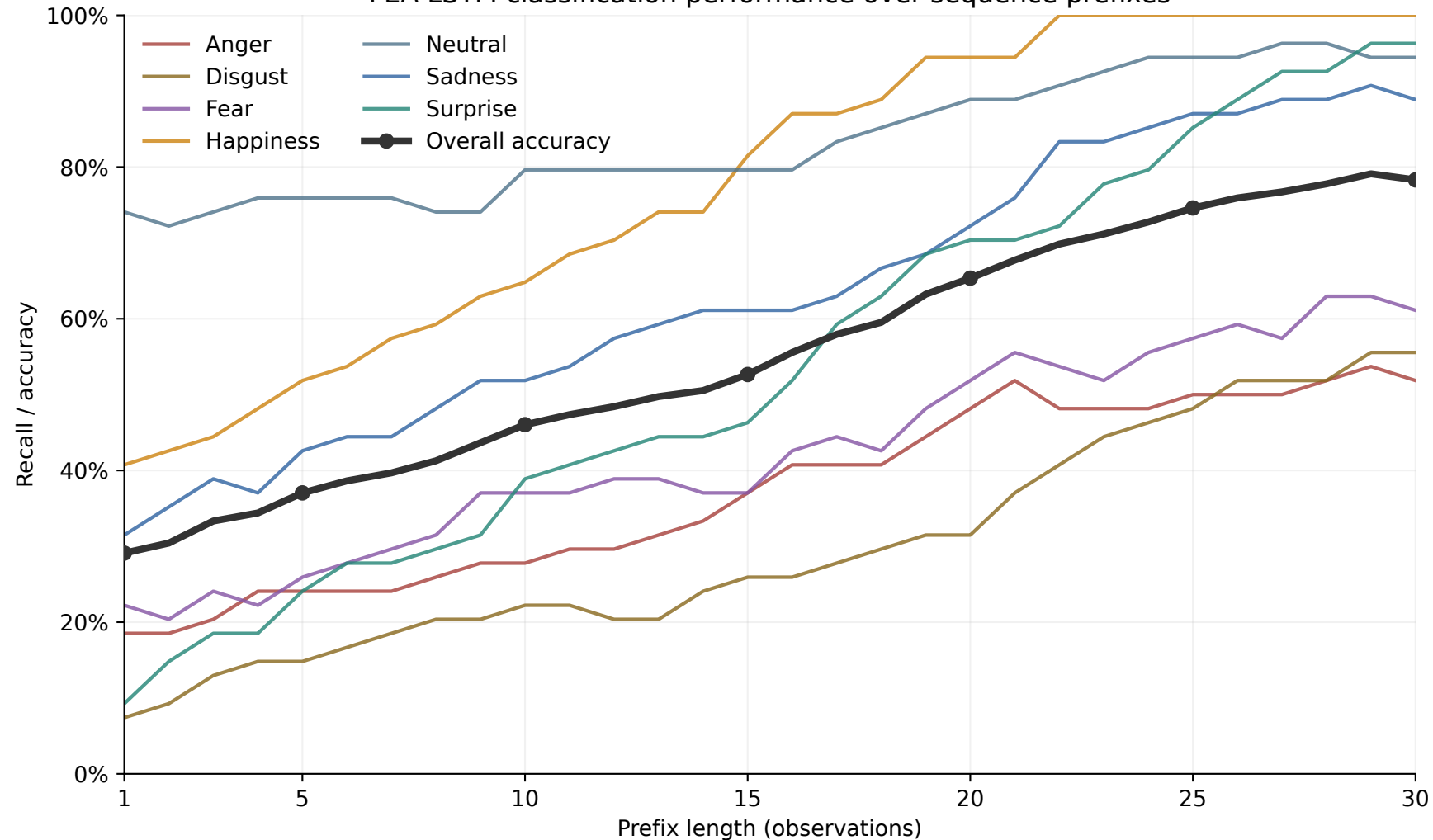
FEA LSTM classification performance over sequence prefixes
