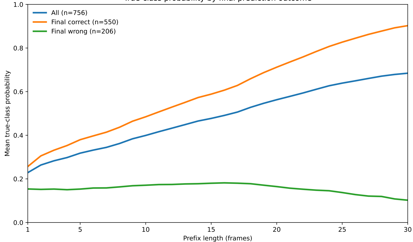
True-class probability by final prediction outcome
