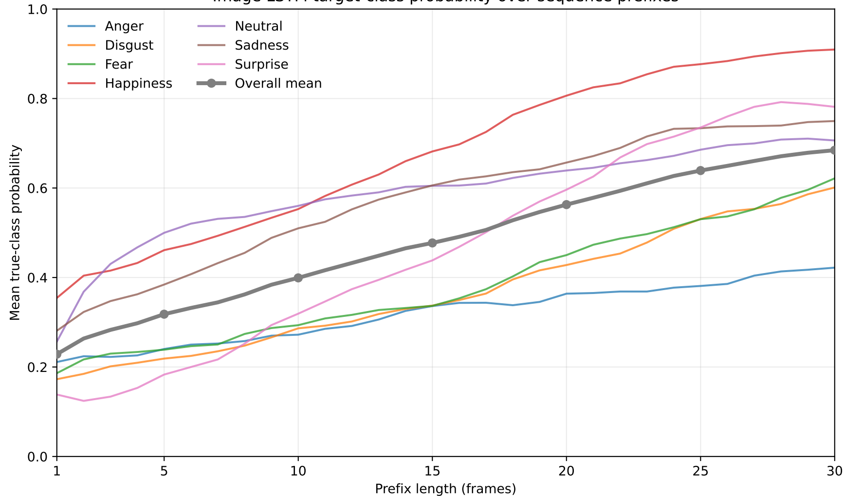
Image LSTM target-class probability over sequence prefixes
