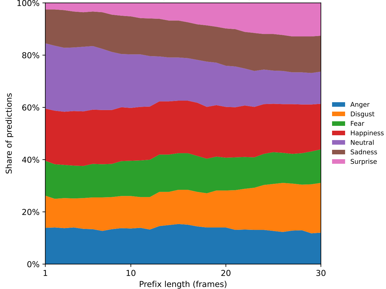
Prediction composition over the prefix
