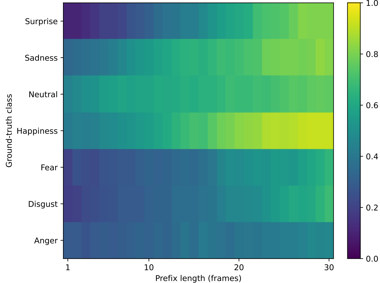
Class recall by prefix length
