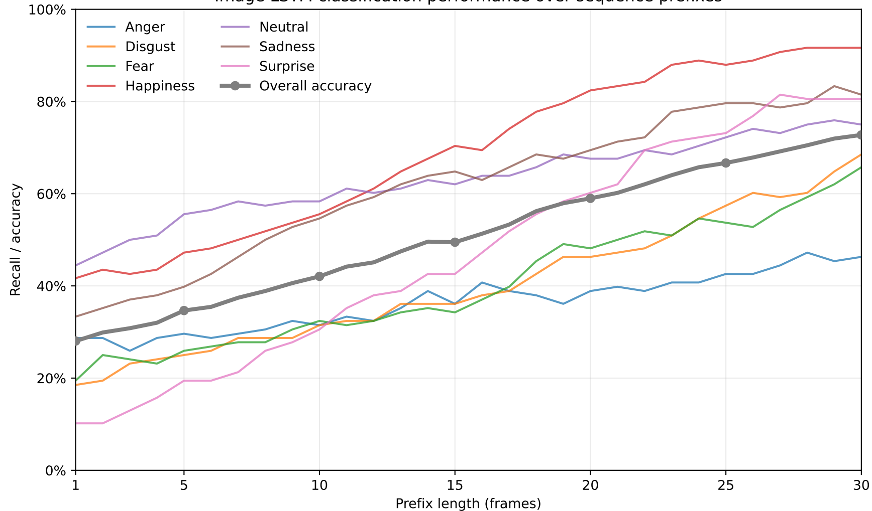
Image LSTM classification performance over sequence prefixes
