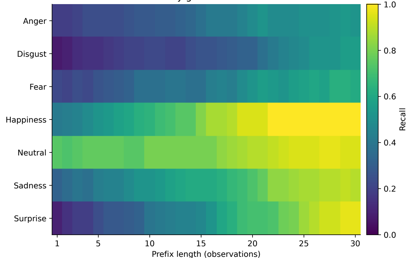
Recall by ground-truth class
