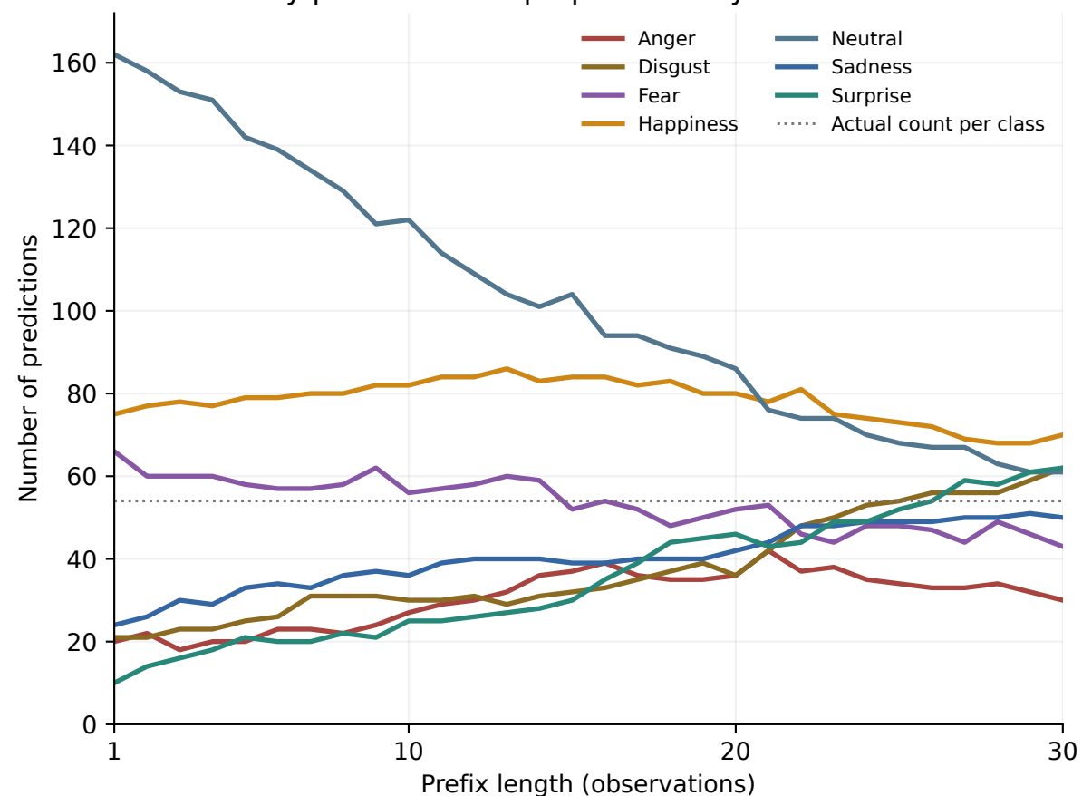
Early predictions disproportionately favor Neutral
