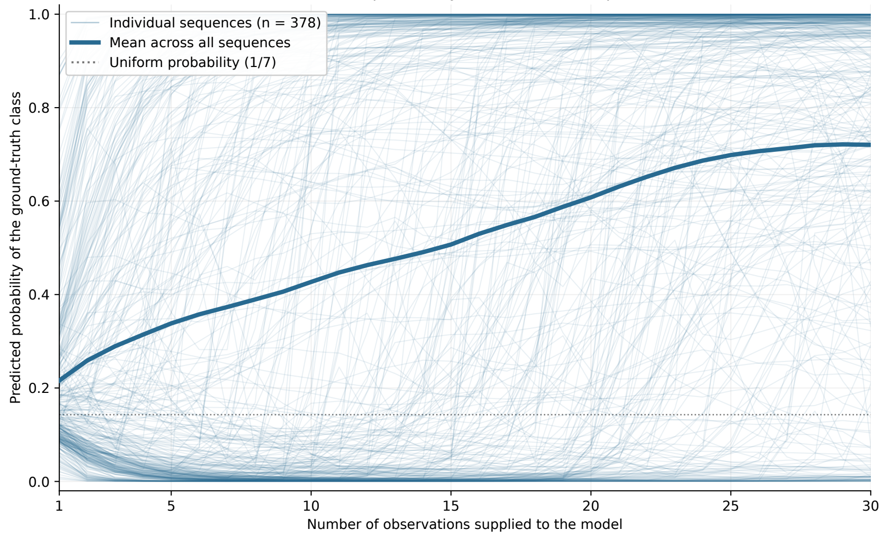
Ground-truth probability across all FEA sequences
