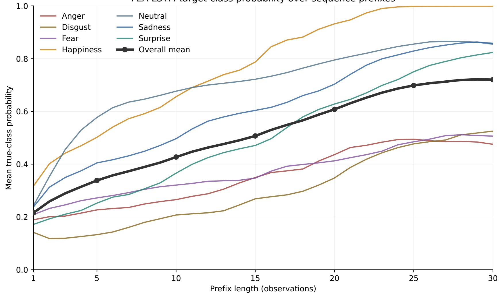
FEA LSTM target-class probability over sequence prefixes
