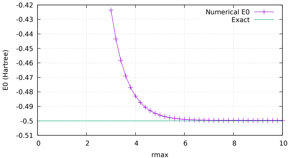
E0 convergence vs rmax ( \Delta r fixed at 0.05)
