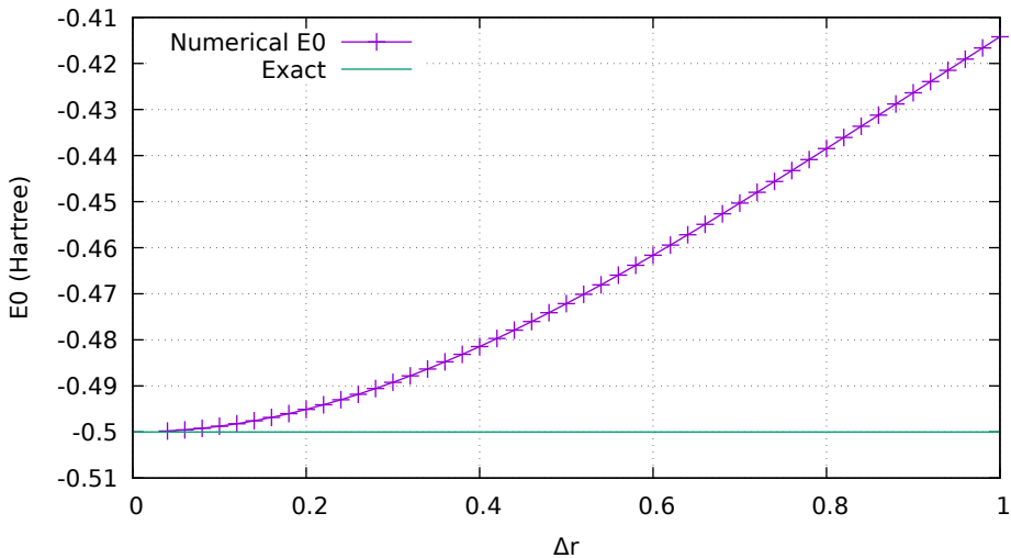
E0 convergence vs \Delta r (rmax fixed at 10.00)
