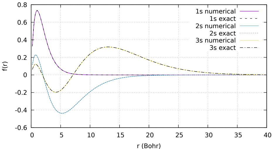
Radial hydrogen s-wave wavefunctions
