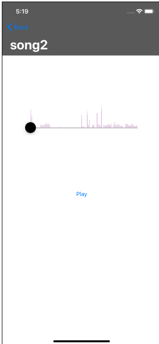
Playback screen
