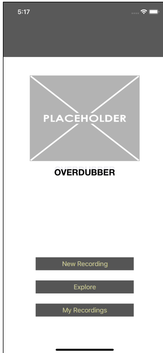
Main Menu
