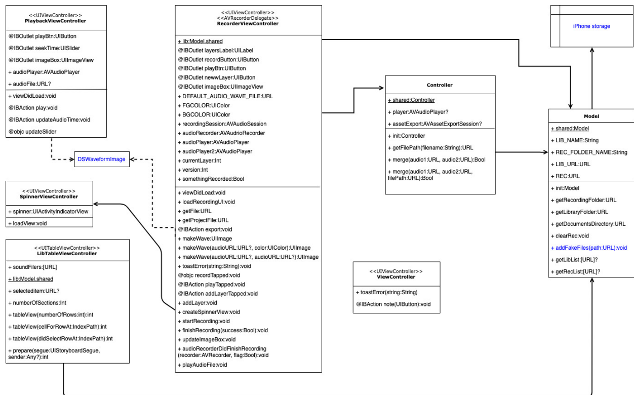
Class Diagram
