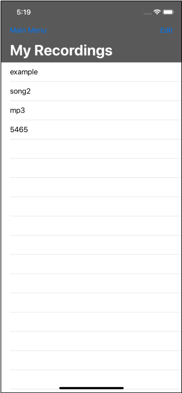
My Recordings
