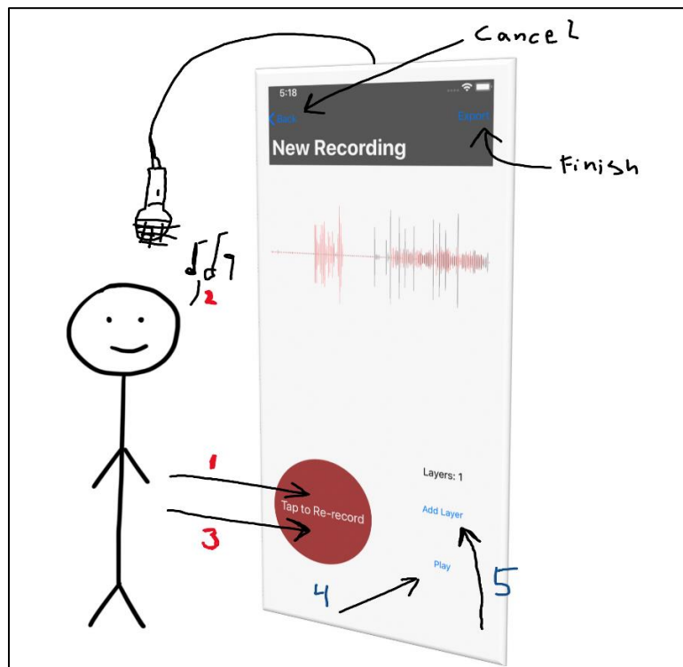
User Interaction
