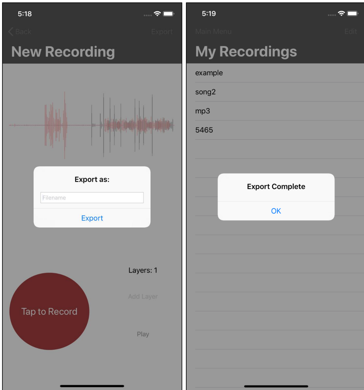
Successful export
