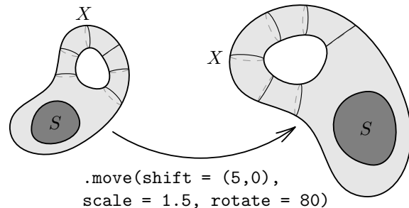
Figure 9: Calling one method to move a smooth object along with its hole, subset, label, and cross sections
