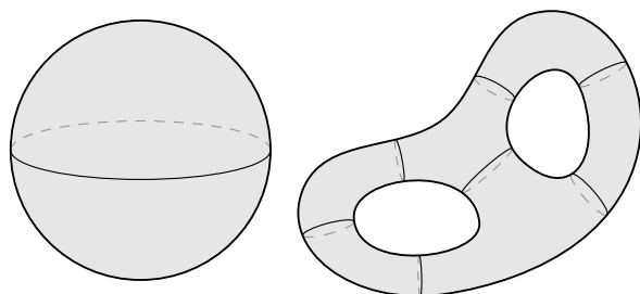
Figure 1: Basic two-dimensional manifolds
