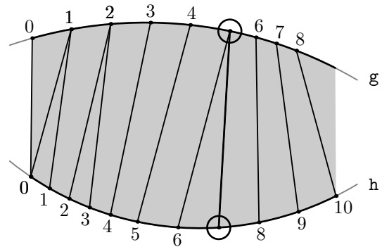
Figure 6: Selecting the optimal section position (circled) within one region
