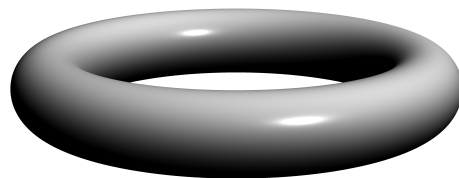
Figure 7: A real 3-dimensional torus
