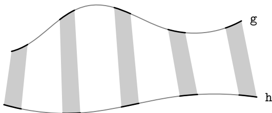
Figure 5: n regions (filled gray) are formed between the paths g and h
