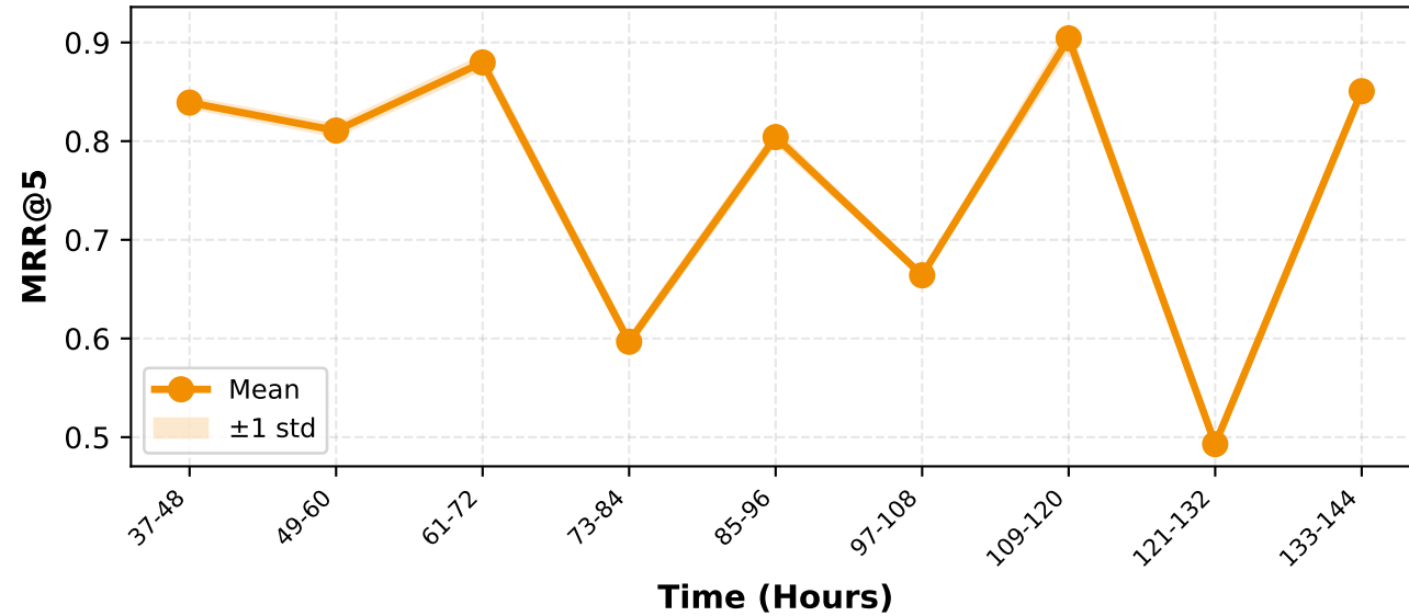
MRR@5 Over Time
