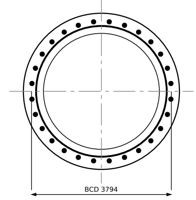
SKIRT BASE / ANCHOR BOLT PLAN 1:100
