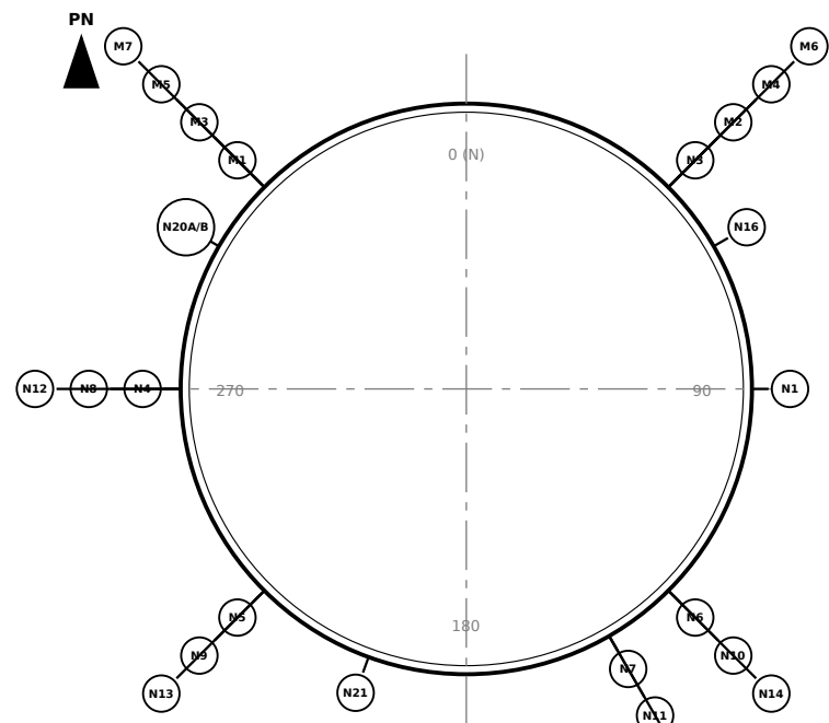
NOZZLE ORIENTATION PLAN 1:100
