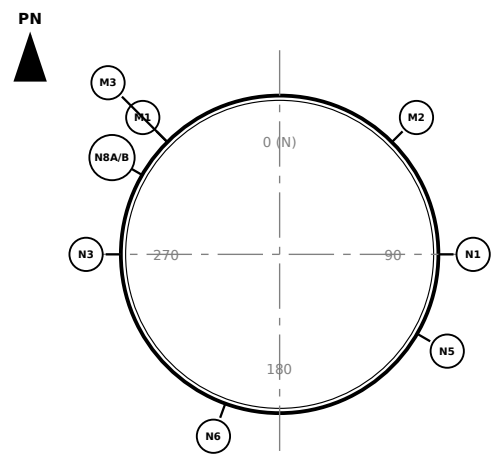
C-105 NOZZLE ORIENTATION 1:50 (manways alternate 315 / 45 deg - platform side)
