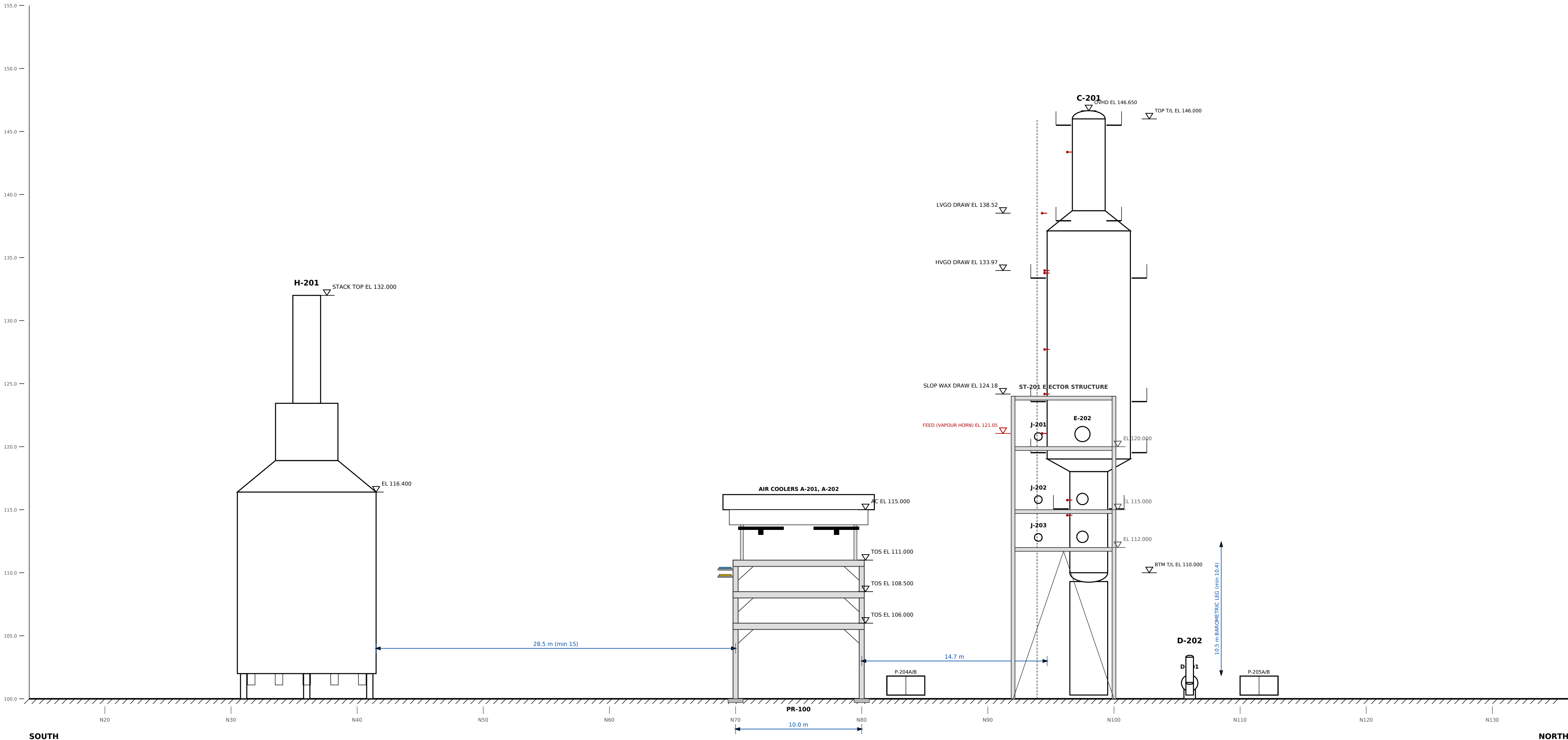
KEY PLAN (NTS) - SECTION PLANE, LOOKING WEST
