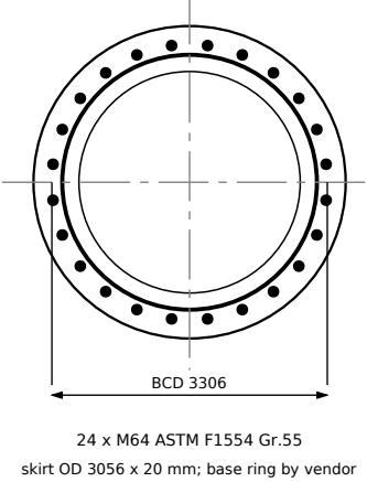
SKIRT BASE / ANCHOR BOLT PLAN 1:100
