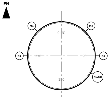
C-103 NOZZLE ORIENTATION 1:50 (manways alternate 315 / 45 deg - platform side)
