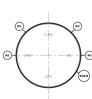
C-102 NOZZLE ORIENTATION 1:50 (manways alternate 315 / 45 deg - platform side)
