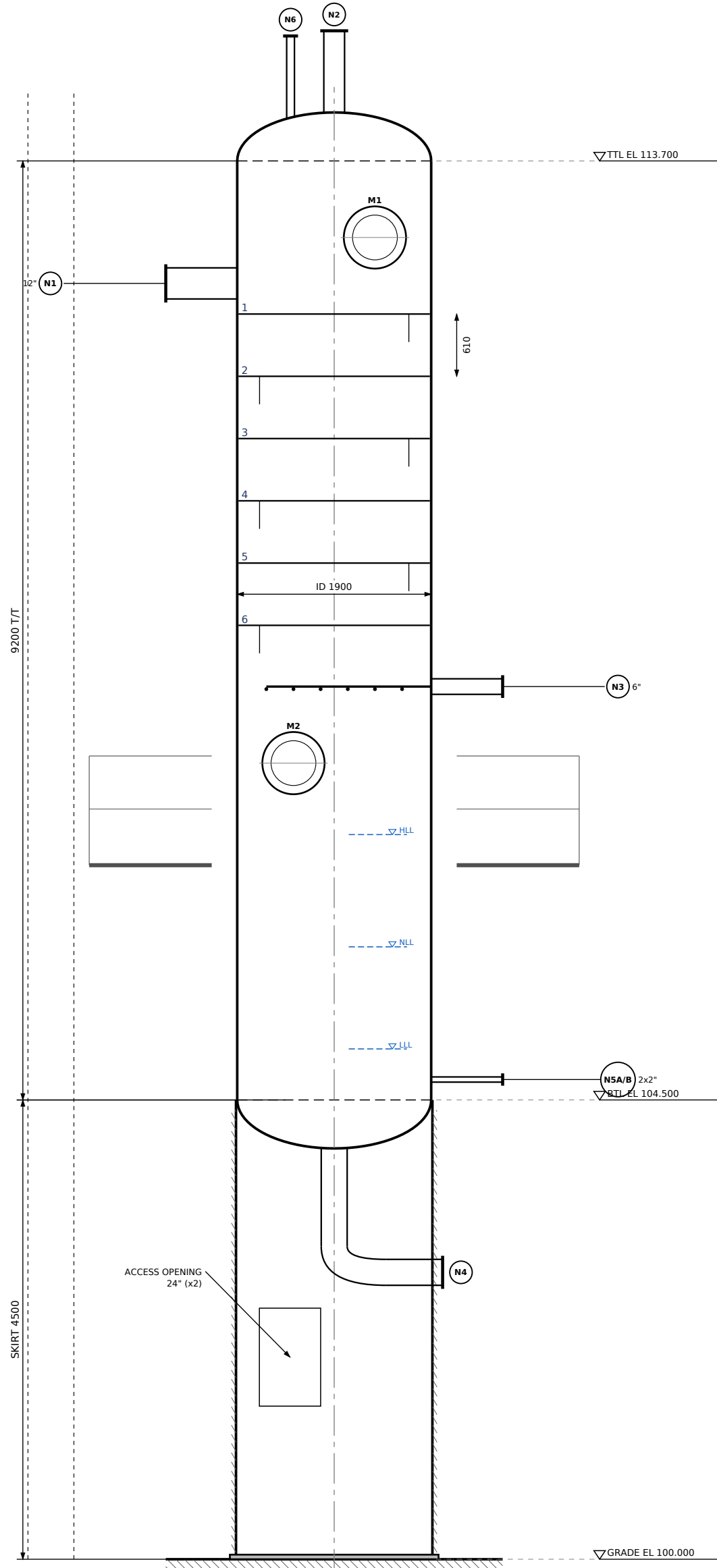
C-103 - DIESEL SIDE STRIPPER ID 1900 x 9200 T/T - ELEVATION 1:50
