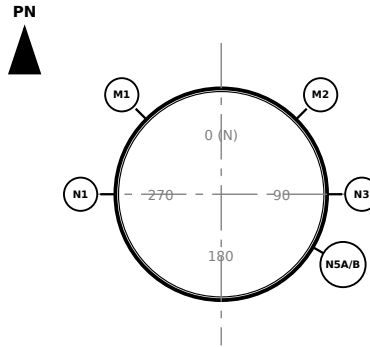
C-104 NOZZLE ORIENTATION 1:50 (manways alternate 315 / 45 deg - platform side)
