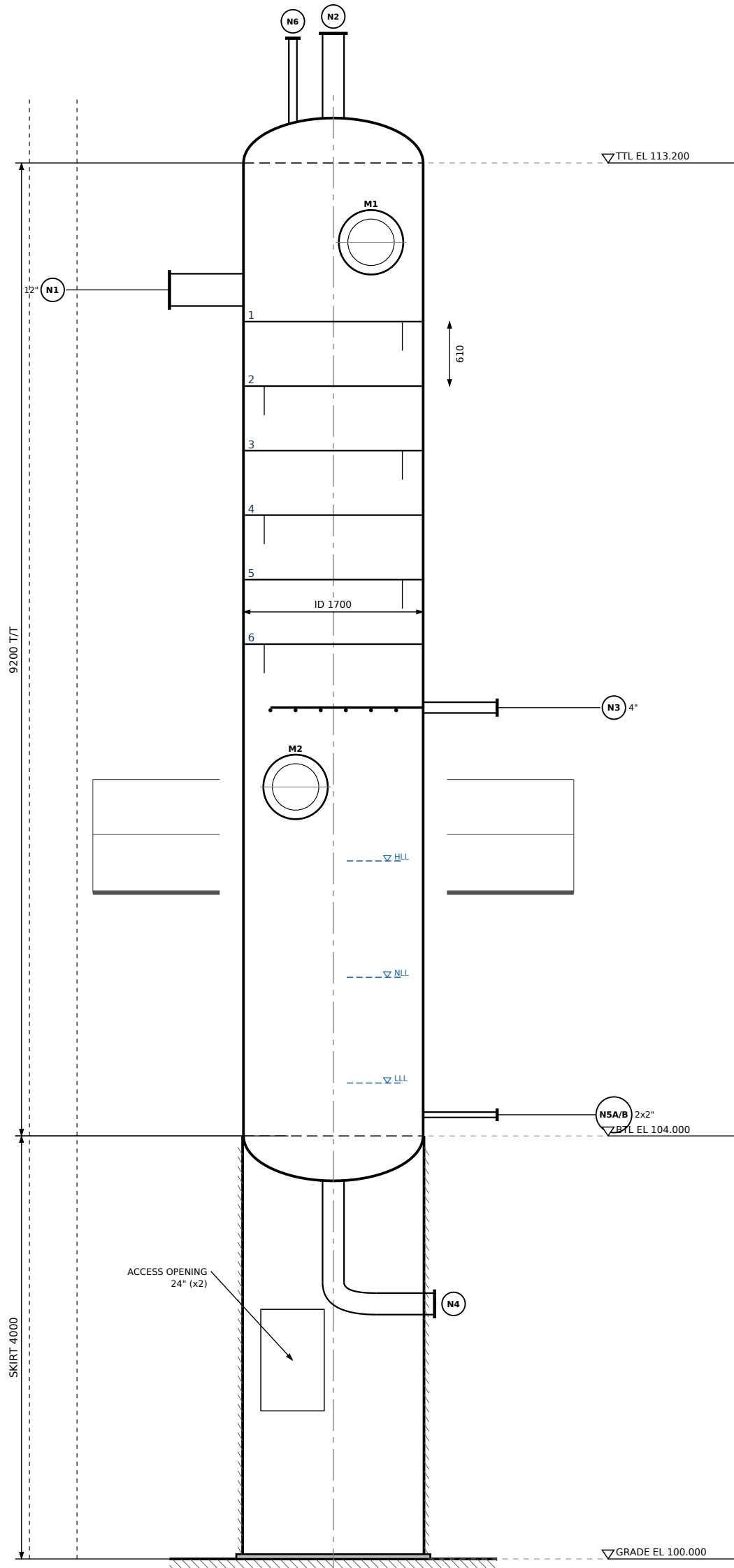
C-102 - KERO SIDE STRIPPER ID 1700 x 9200 T/T - ELEVATION 1:50
