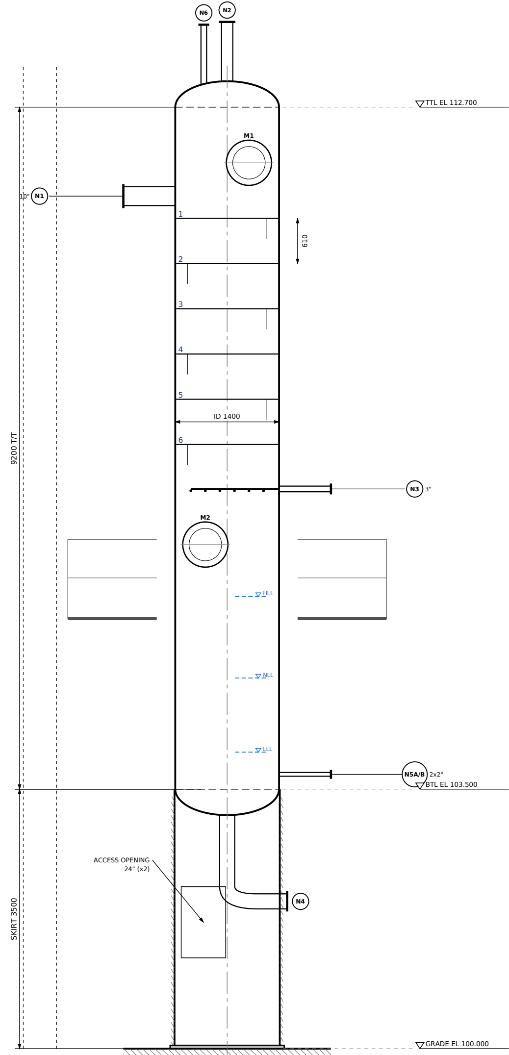
C-104 - AGO SIDE STRIPPER ID 1400 x 9200 T/T - ELEVATION 1:50
