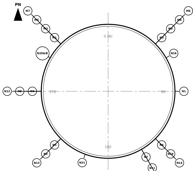
NOZZLE ORIENTATION PLAN 1:100 (manways alternate 315 / 45 deg - platform side)
