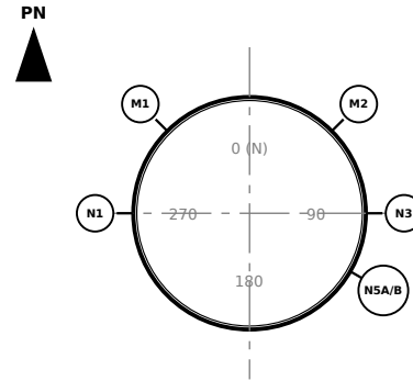
C-104 NOZZLE ORIENTATION 1:50 (manways alternate 315 / 45 deg - platform side)
