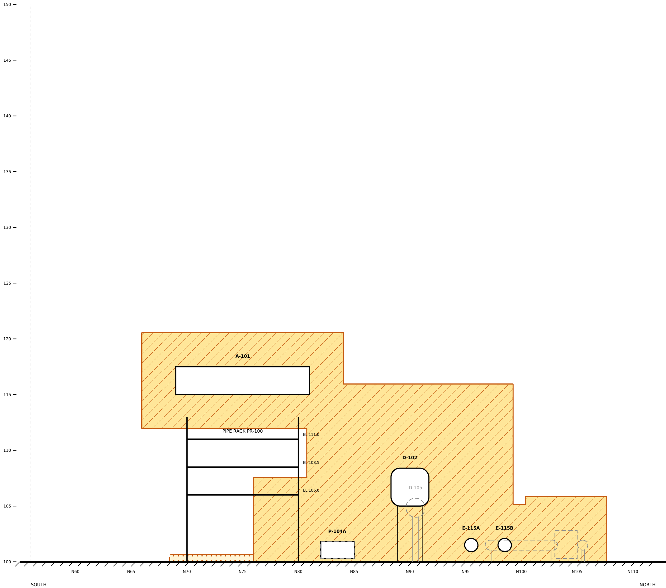
SECTION A-A (cut at E 79, looking west) SCALE 1:200
