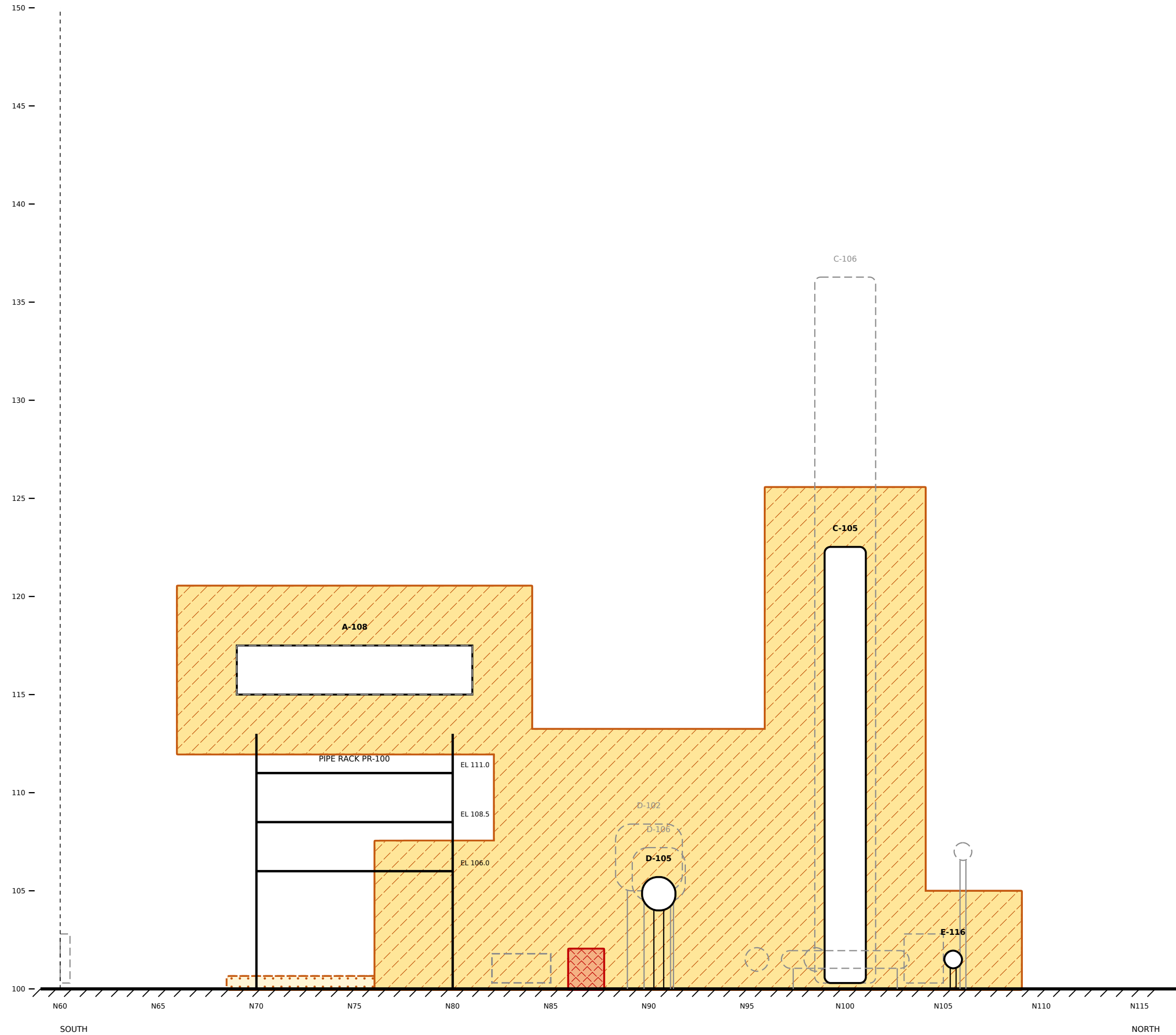
SECTION B-B (cut at E 64, looking west) SCALE 1:200
