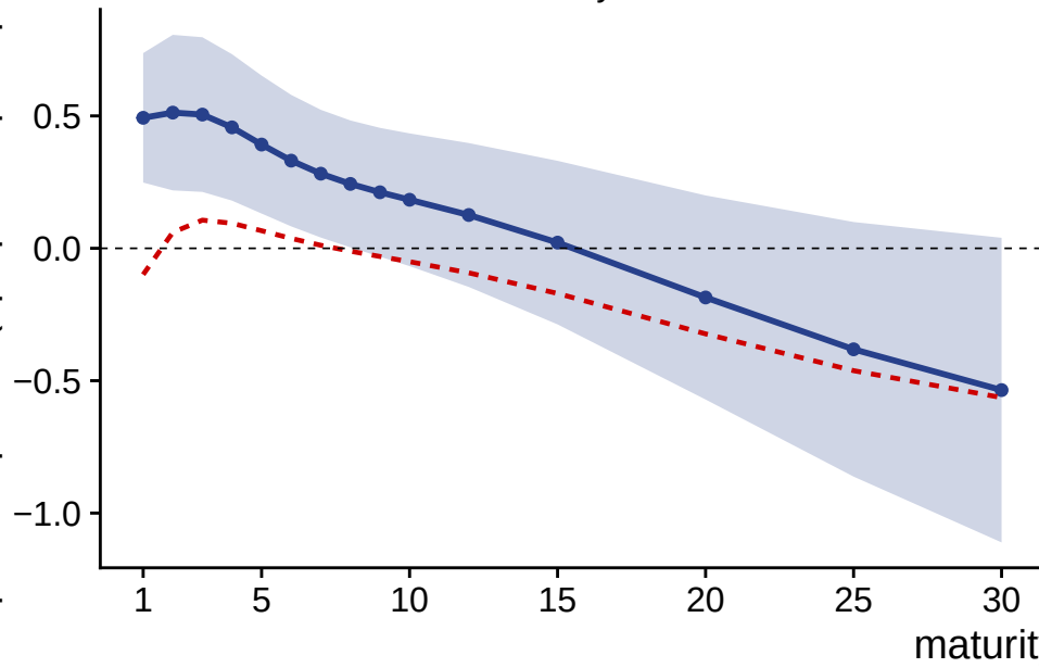
Nominal yields
