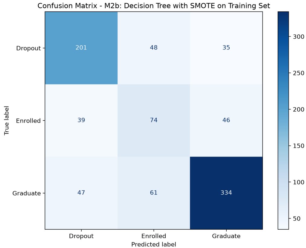
Figure 13: Confusion matrix of M2b (SMOTE on the training set only) on the same 885-sample held-out test set. The model correctly classifies 201/284 Dropout , 74/159 Enrolled , and 334/442 Graduate students – an improvement over both M0 and M2a on every class except a marginal reduction on Graduate .
