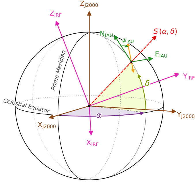
Figure 1: A diagram depicting the relation between J2000 and IRF and the definition of Polarization Angle in the celestial frame. The three basis vectors of J2000 are shown in brown, the source direction ( \alpha , \delta , and its projection into the XY plane) is shown by the dotted red lines. The IRF basis vectors are shown in magenta, the Z-axis here marks the instrument pointing direction. The green vectors show the local (with respect to the celestial North pole) North and East in the tangent plane perpendicular to the source direction. The orange line marks the projection of the electric field vector and the polarization angle is defined as \psi_{IAU} .
