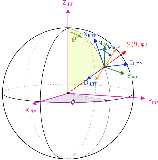
Figure 2: A diagram showing the relation between IRF and ILTP and definition of polarization angle in the ILTP. The IRF basis vectors are shown in magenta and the source direction in IRF ( \theta, \phi , and its projection into the XY plane) is shown by the dotted red lines. The ILTP basis vectors are shown in blue. As before, IRF Z-axis direction corresponds the pointing direction of the instrument. The Z-axis of ILTP points in the direction opposite to the source (i.e. the direction of incoming photons). The X and Y axis of ILTP are the local (with respect to instrument North, i.e. the pointing direction) North and East. The orange line marks the projection of electric field vector and the Polarization Angle in ILTP is defined by \psi_{LTP}
