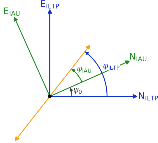
Figure 3: Projected view of the tangent plane perpendicular to the source direction as seen from the source. The orange line is the projected electric field vector. As defined by the IAU convention the \psi_{IAU} is measured from the local North increasing positively towards the East. The \psi_{ILTP} is defined in a similar way but with respect to the ILTP North and East. The angle \psi_0 shows the relative offset between the two frames.
