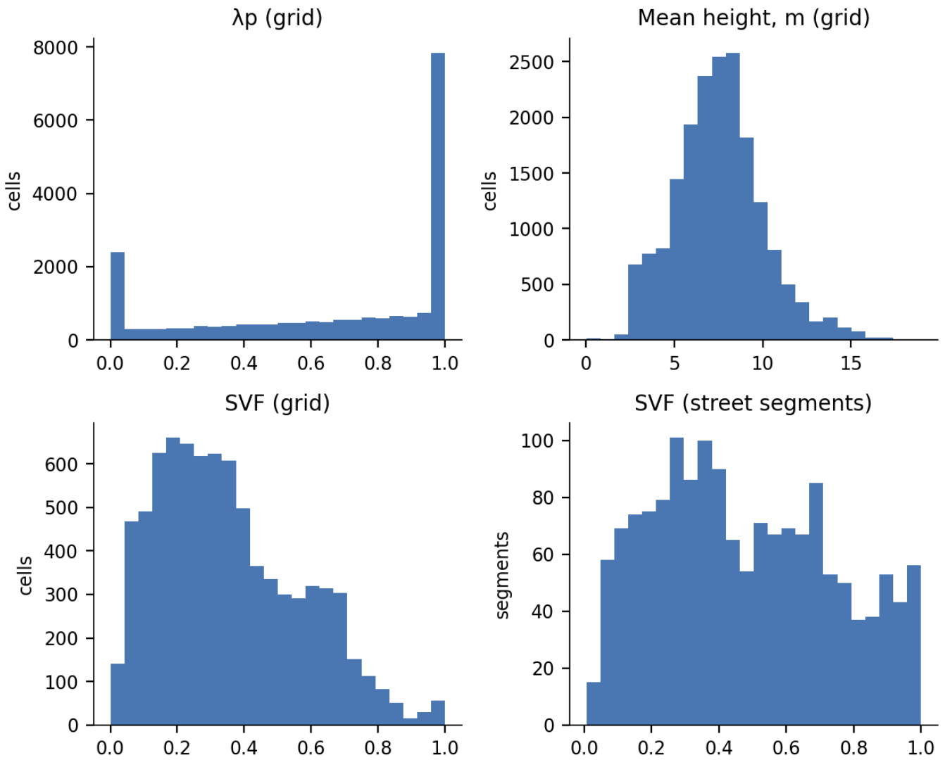
Figure 2. Distributions of \lambda_p , mean height, SVF (grid), and street-level SVF (segments) across Maré, as histograms.
