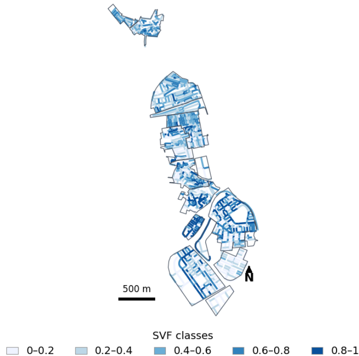
Figure 3. Sky View Factor by street segment, five discrete classes with class edges in the legend. No basemap, no coordinates.
