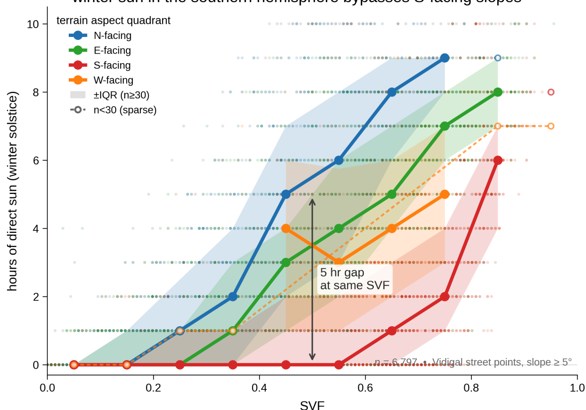
Figure 6. Per-quadrant median solar hours as a function of SVF, on Vidigal's sloped cells (slope \geq 5^\circ , n = 6,797 along-street points). The four traces — one per terrain-aspect quadrant (N / E / S / W) — do not collapse onto a single curve. At a fixed SVF \approx 0.5 , an N-facing cell receives \approx 5 hours of direct sun on the winter solstice while an S-facing cell receives \approx 0 ; the same is true at SVF \approx 0.7 (8 hr vs 2 hr). Shaded bands show the inter-quartile range; trace segments where the SVF bin contains fewer than 30 cells are dashed (open markers) to flag the small-sample tails (W-quadrant beyond SVF \approx 0.65 ). Underlay scatter is the full set of sample points coloured by aspect bearing, making the cloud's directional structure visible.
